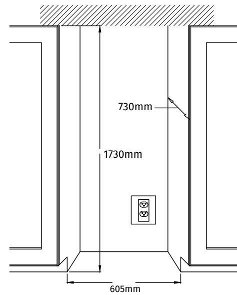
CABINET CUT-OUT
