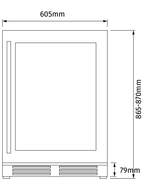
CABINET CUT-OUT
