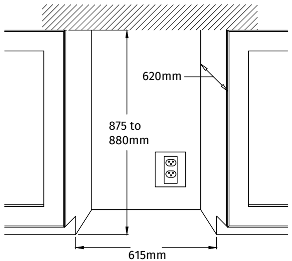
CABINET CUT-OUT
