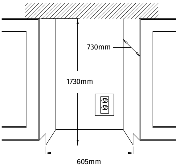
CABINET CUT-OUT
