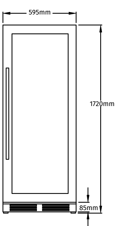
CABINET CUT-OUT
