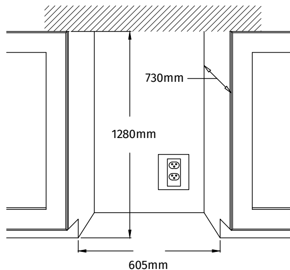
CABINET CUT-OUT
