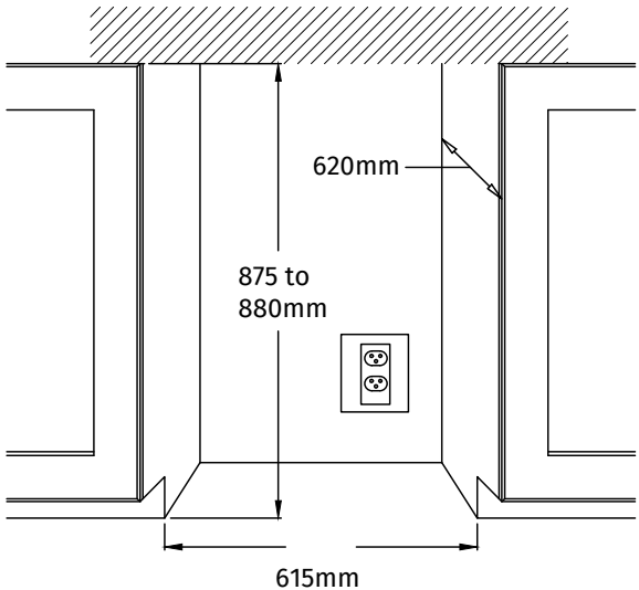
CABINET CUT-OUT
